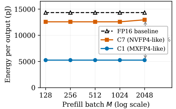
Fig. 3. Per-output energy of FP16 / C7 / C1 on LLM prefill across M \in \{128, \dots, 2048\} . All three configurations are nearly M -invariant, consistent with the cost decomposition of Sec. IV-D; the C1-vs-C7 gap stays at 58–59% over the entire range. VLM and VLA prefill scans are future work.
